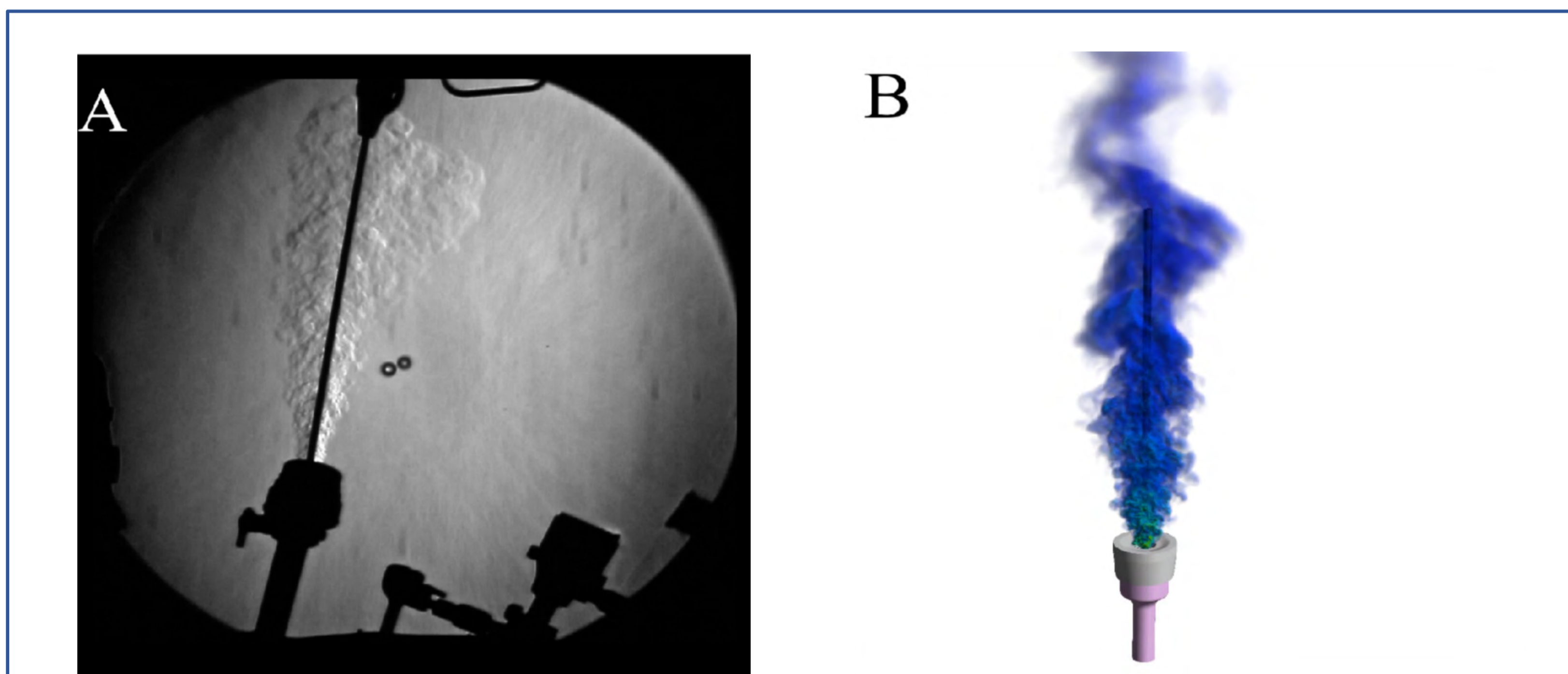
Figure A shows a Schlieren image of gas leaking out of a surgical port. Figure B shows a CFD simulation of the leak (Crowley et al., 2021, p. 5). Schlieren imaging is a useful visual aid that can be used in the surgical theater however, it does not show the individual particles needed to analyze. The laser used in PIV solves this issue.
